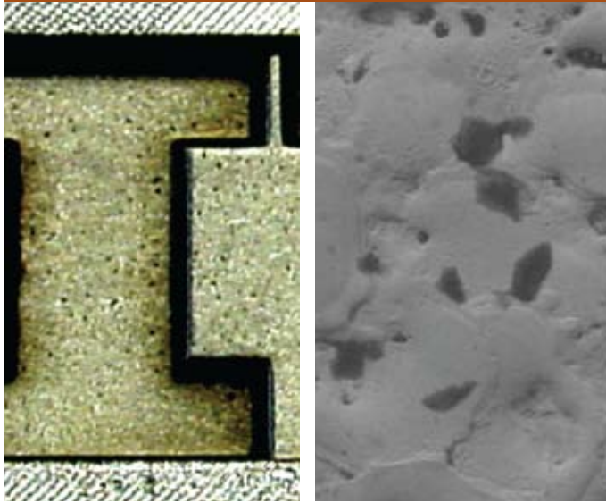
Cavity EDMed with an electrode exhibiting an inconsistent microstructure.
