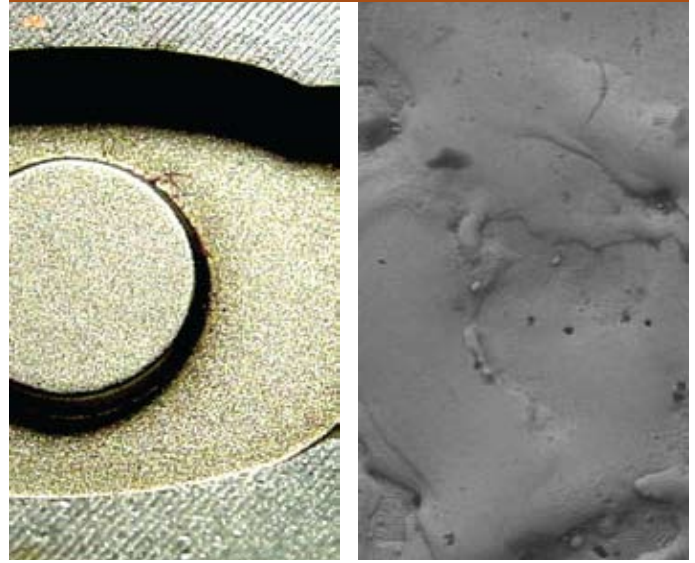
Cavity EDMed with an electrode exhibiting a consistent microstructure.
